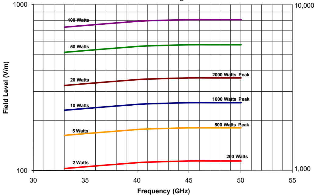
ATH33G50 Field Strength at 1 meter
