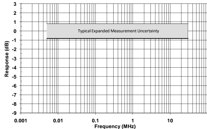
FL7030CC Typical Calibrated Frequency Response (with correction factors applied)
