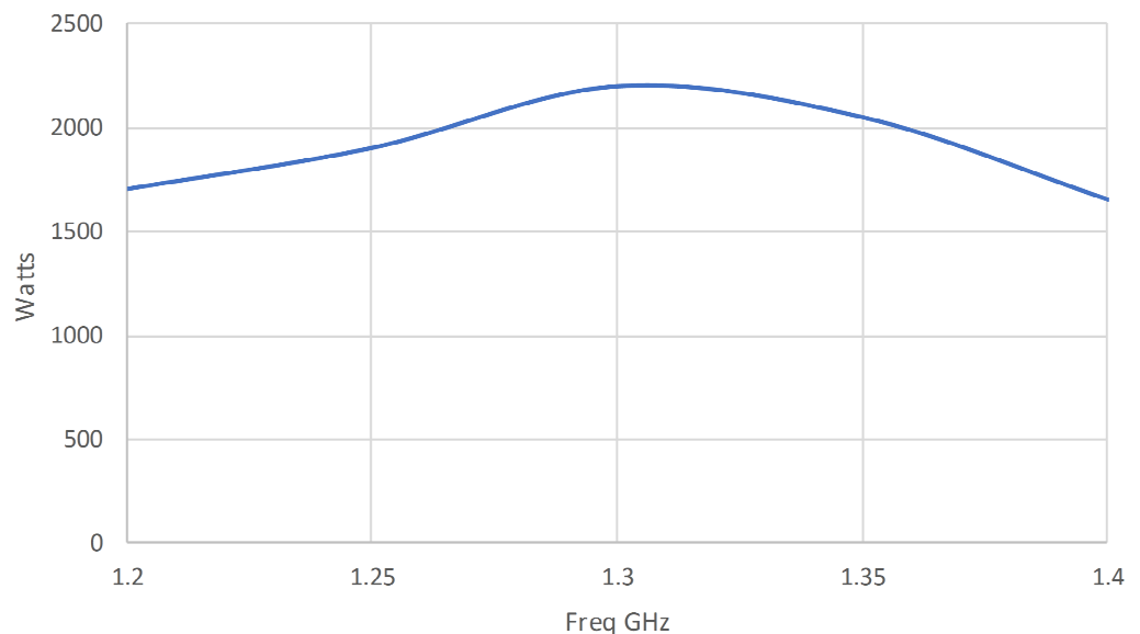
1500SP1z2G1z4 Typical Power Output
