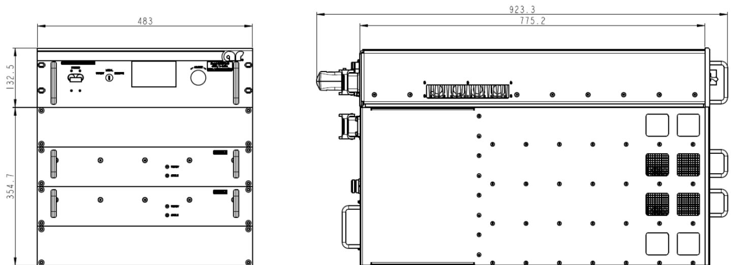
Units=mm; base model 12000SP1z2G1z4 shown
